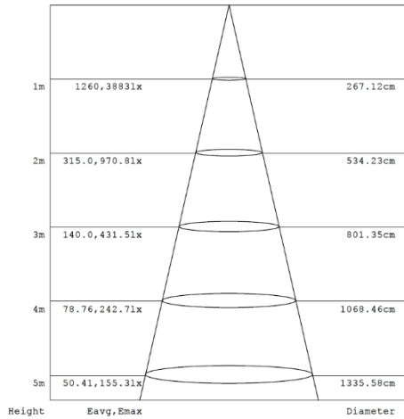
Diagram for RSUF966FT-24 in 5000K. Other diagrams available on request
