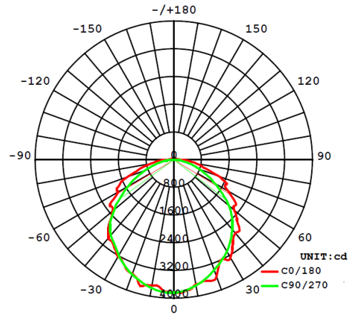
Diagram for RSUF966FT-24 in 5000K. Other diagrams available on request
